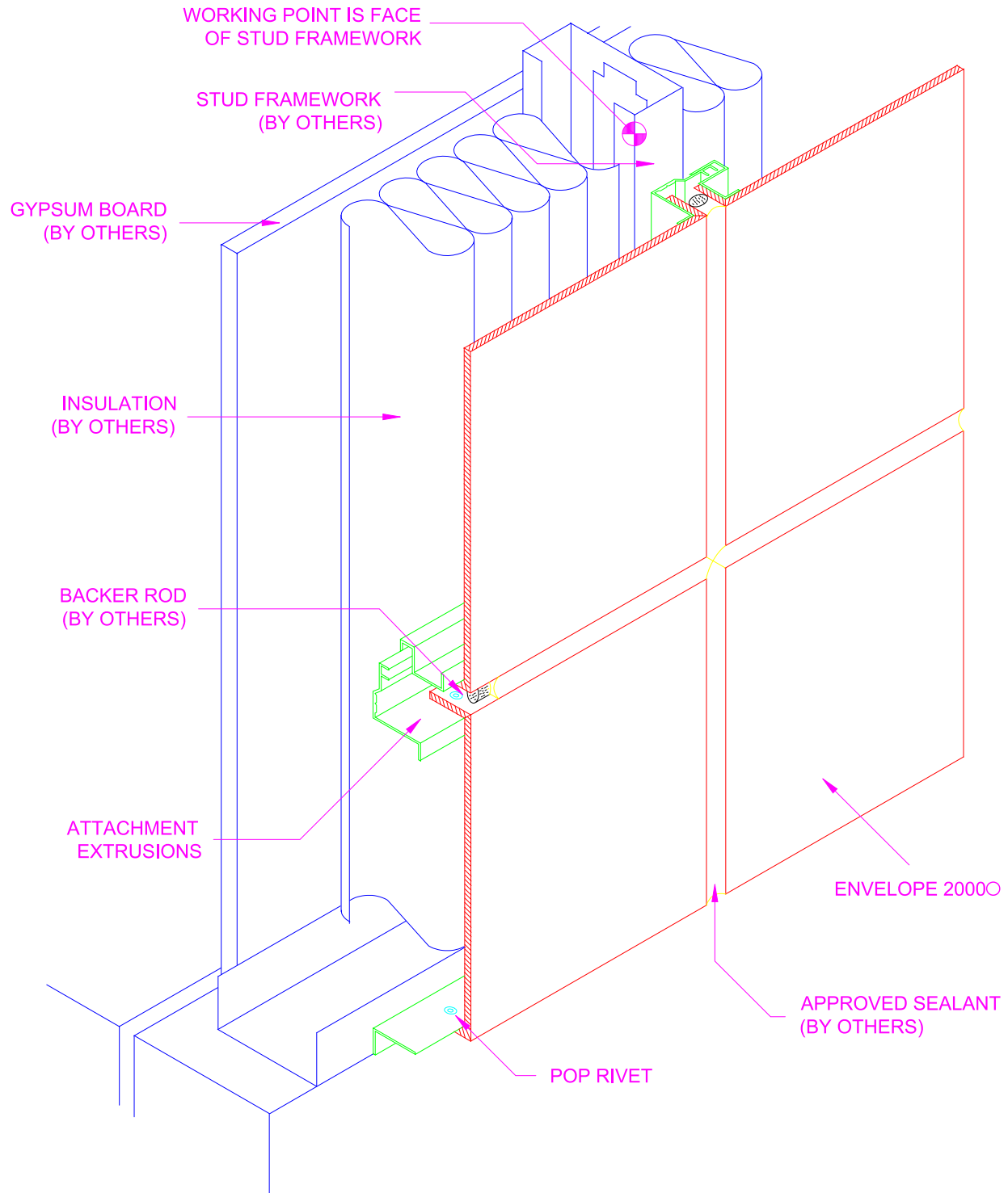
1 SYSTEM ISOMETRIC
