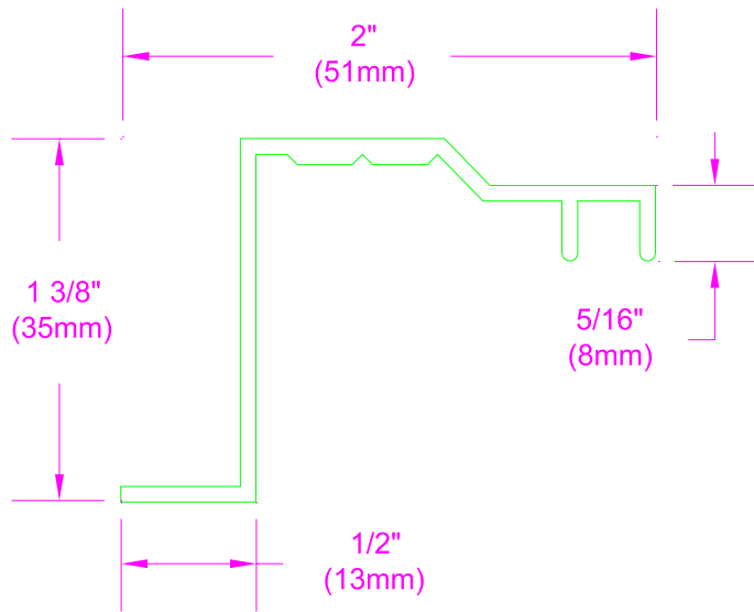
RR-121 MALE ANGLE
