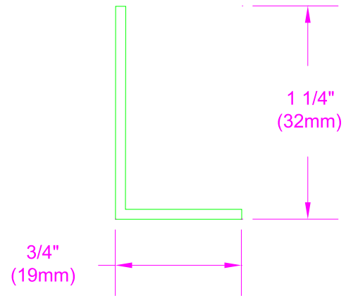
RR-104 END RUN ANGLE
