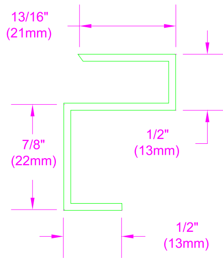
RR-122 FEMALE ANGLE
