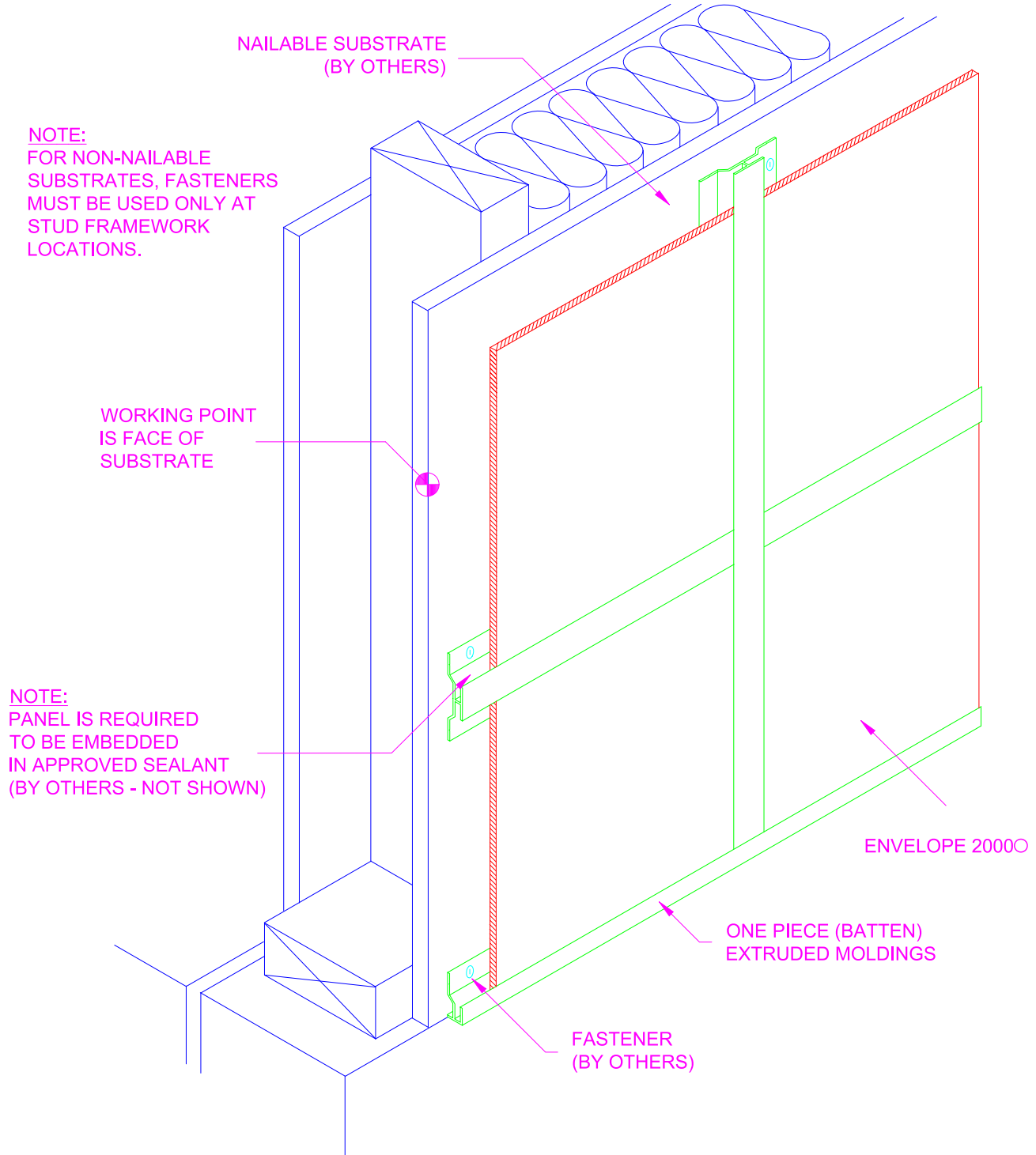
1A SYSTEM ISOMETRIC, OPTION 1
