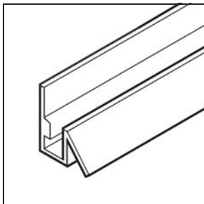
E-305 DRIP EDGE Face Leg: 1/2" (13mm) Height: 1" (25mm) Length: 12' (3658mm)
