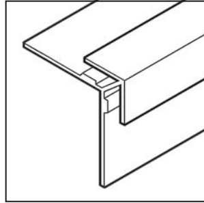
E-302 O/S CORNER Face Leg: 3/4" (19mm) Width: 2" (51mm) Length: 12' (3658mm)
