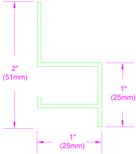
PA-3X WATER TABLE
