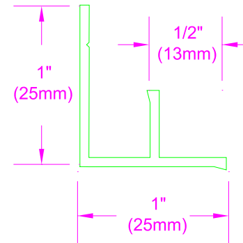
PA-9X INSIDE CORNER
