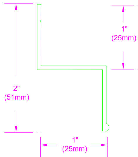
PA-4X HORIZONTAL
