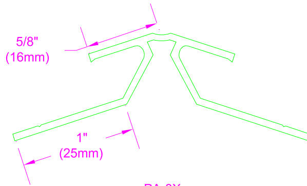
PA-8X OUTSIDE CORNER
