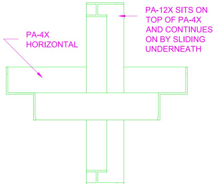
15B HORIZONTAL ONLY, OPTION 2
