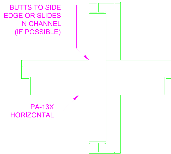
15A HORIZONTAL ONLY, OPTION 1
