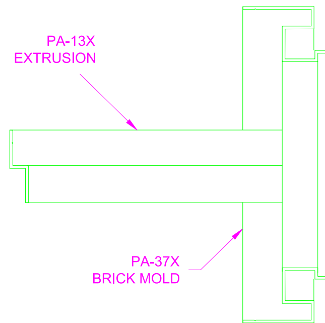
17B HORZ TERMINATION ONLY, OPTION 2
