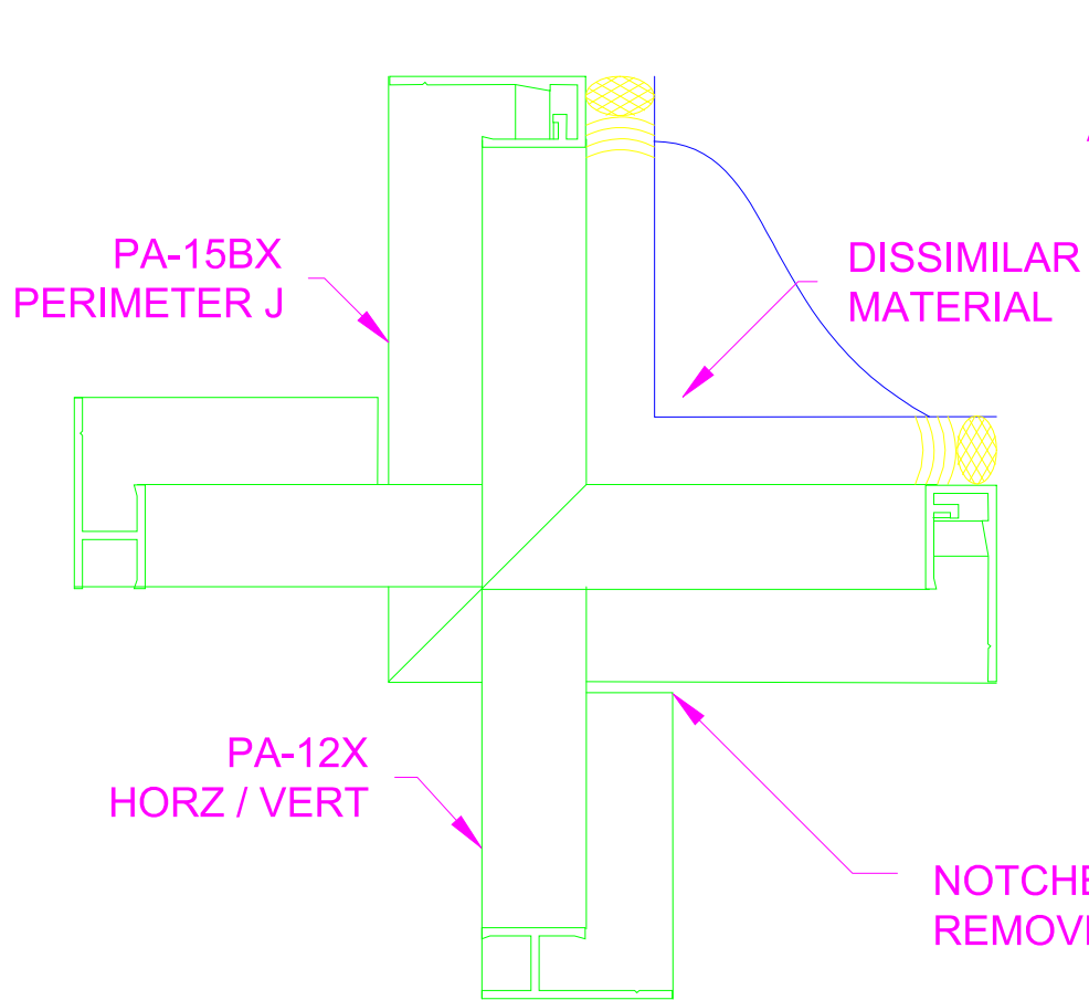
20A DISSIMILAR MATERIAL CORNER, OPT. 1
