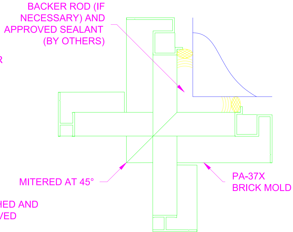
20B DISSIMILAR MATERIAL CORNER, OPT. 2
