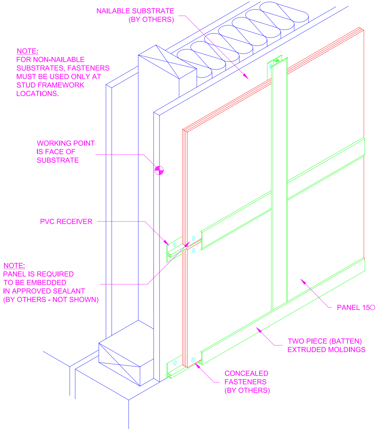
1A SYSTEM ISOMETRIC, OPTION 1
