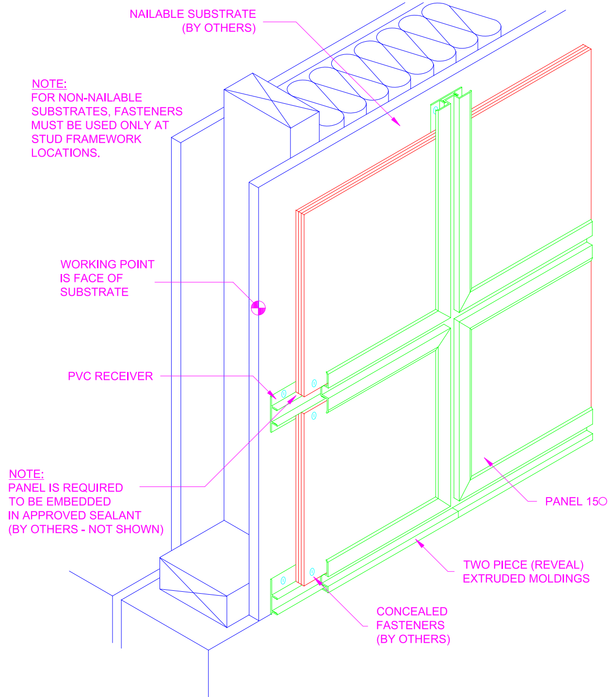
1B SYSTEM ISOMETRIC, OPTION 2
