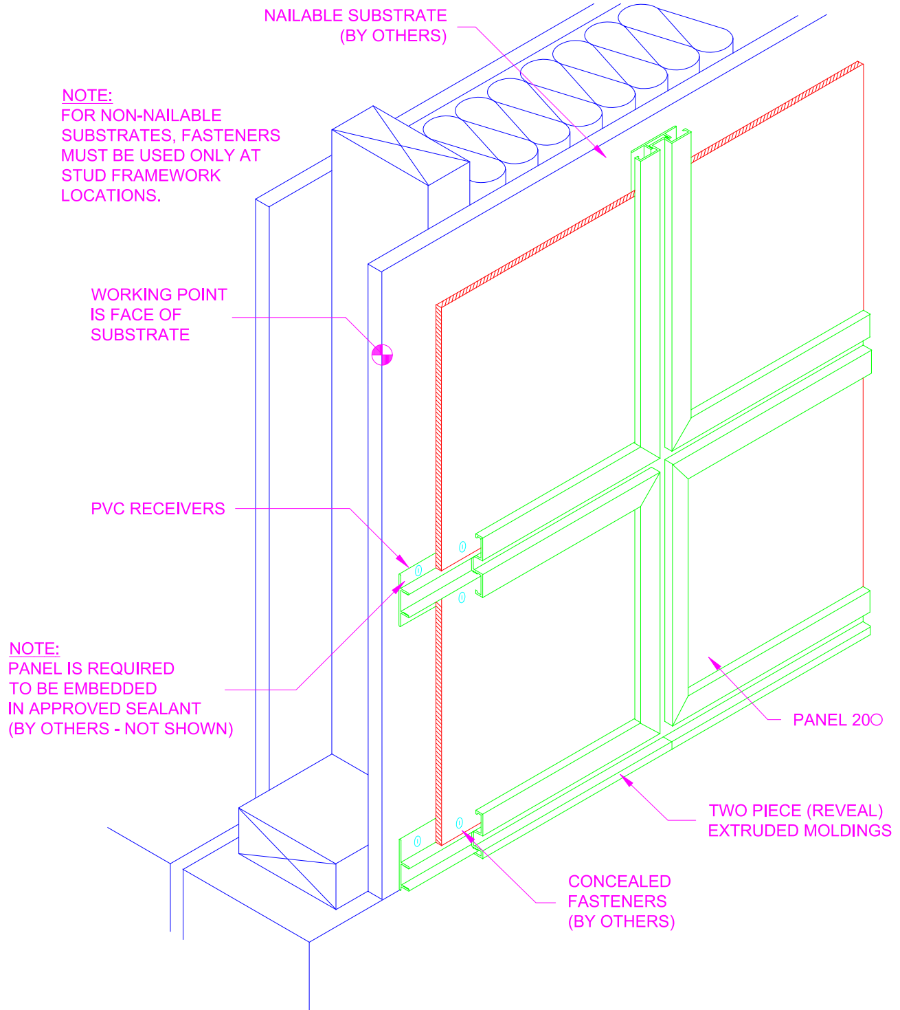
1B SYSTEM ISOMETRIC, OPTION 2
